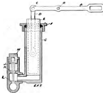
FIG. 188.—Section of a Type of Plunger Feed Pump. As is obvious, the valve opened by suction of the up-stroke is closed by compression of the down-stroke, and vice versa . This pump is equipped with a double, or compound, valve, which, as may be seen, secures perfect balance in operation with the simplest possible constructions. The stem of the suction valve enters a bore in the stem of the outlet valve. Referring to the lettered parts: A is the pivoted lever working the pump from the crosshead of the engine; B, the fulcrum point; C, the attachment of the piston rod; D; E, the trunk plunger; F, the packing cap; G, the pump cylinder; H, nut on the valve chamber port; J, the valve chamber; K, water outlet valve; L, water inlet valve.
